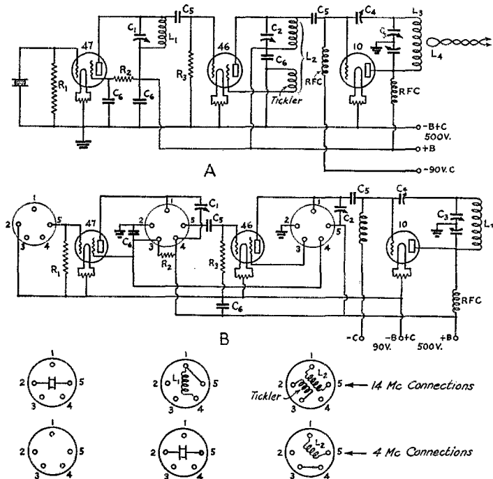
FIG. 1—(A) R. F. EXCITER CIRCUIT AND (B) COIL CONNECTIONS L_1, L_2, L_3, L_4 — See coil table C_1, C_3 —33 \mu f.d. midget variable condensers C_2 — Double 35- \mu f.d. double-spaced midget C_4 — Double-spaced 25- \mu f.d. midget C_5 — 0.001- \mu f.d. mica C_6 — 0.002- \mu f.d. mica R_1 — 25,000-ohm 1-watt R_2 — 50,000-ohm 5-watt R_3 — 30,000-ohm 1-watt
