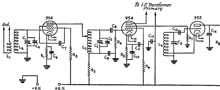
FIG. 1—WIRING OF THE ACRN INPUT UNIT OF THE SUPERINFRAGENERATOR RECEIVER
