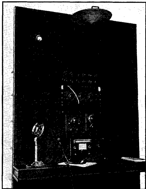
THE RECEIVER AND OTHER STANDARD PIECES OF EQUIPMENT ARE MOUNTED BEHIND CUT-OUTS IN THE PLY-WOOD PANELS, WHILE THE JACK-STRIP PROVIDES PLENTY OF PATCHING CONNECTIONS FOR THAT DESIRABLE FLEXIBILITY
